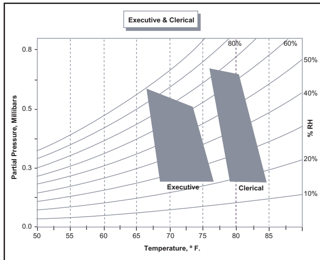
Figure 4. PMV Chart
