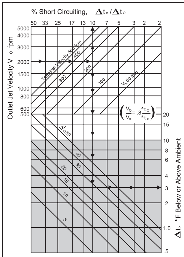
Figure 39. Temperature Differential and Short Circuiting
