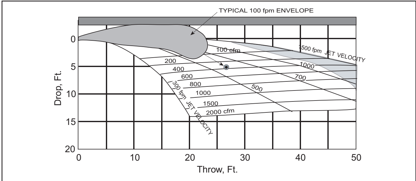
Figure 12. Throw and Drop for Outlet 1 Foot Below Ceiling 0 Degree Deflection, 0 Degree Spread
