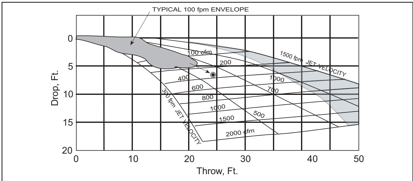
Figure 13. Throw and Drop for Outlet Without Ceiling, 0 Degree Deflection, 0 Degree Spread
