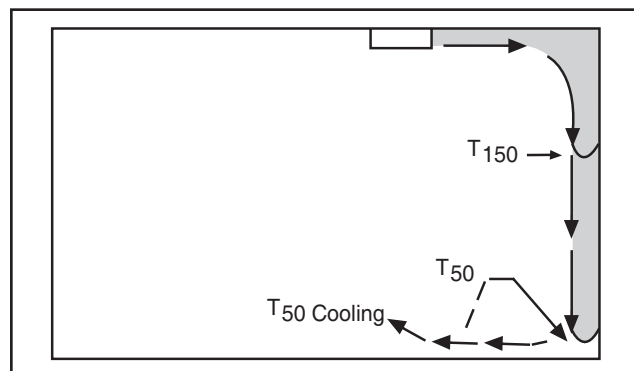
Figure 33. Cooling with Outlet Located Near Perimeter Wall
